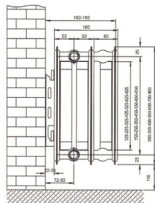
TF TRIPLE PANEL TRIPLE CONVACTOR
